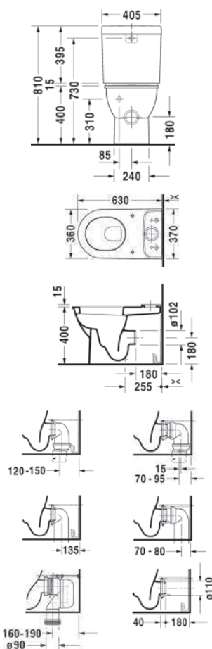
s/trap 305 mm toilet 212301 one-piece
