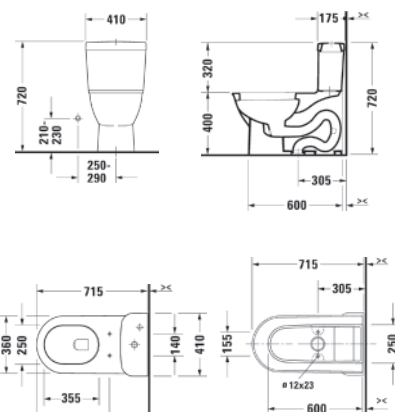
s/trap 305 mm toilet 212301 one-piece
