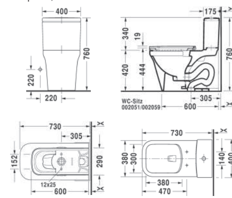
s/trap 305 mm toilet 217501 one-piece, rimless soft-close seat (option) 002059
