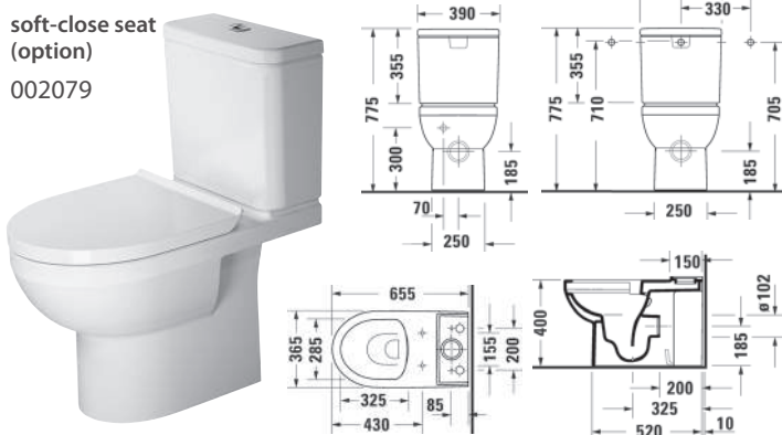
toilet 218309 p/trap, rimless
