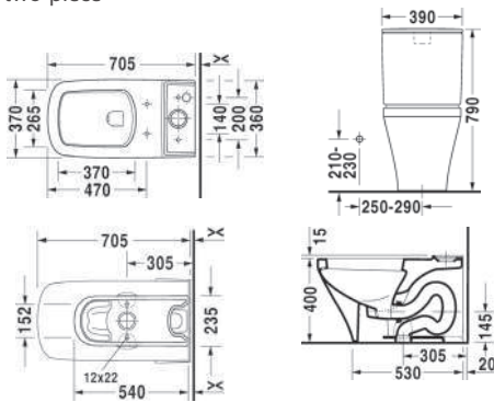
s/trap 305 mm toilet 216001 two-piece
