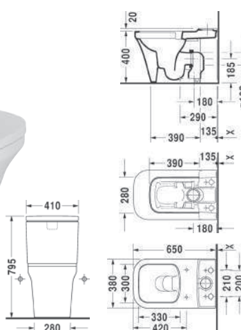
toilet 216709 vario outlet rimless soft-close seat (option) 002049
