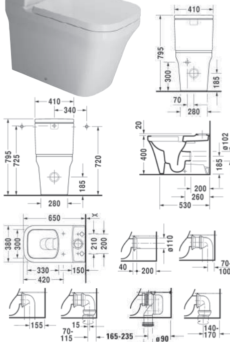
toilet 216709 vario outlet rimless soft-close seat (option) 002049
