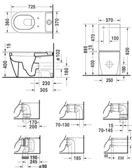
toilet 212909 vario outlet soft-close seat (option) 006339
