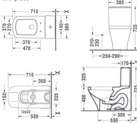
s/trap 305 mm toilet 215701 two-piece
