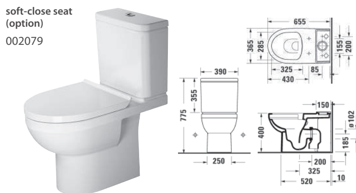
toilet 218301 s/trap, rimless
