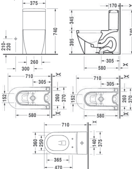
s/trap 305 mm toilet 213301 one-piece soft-close seat (option) 006339
