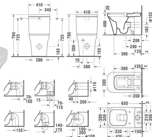
toilet 216309 vario outlet, rimless soft-close seat (option) 002049
