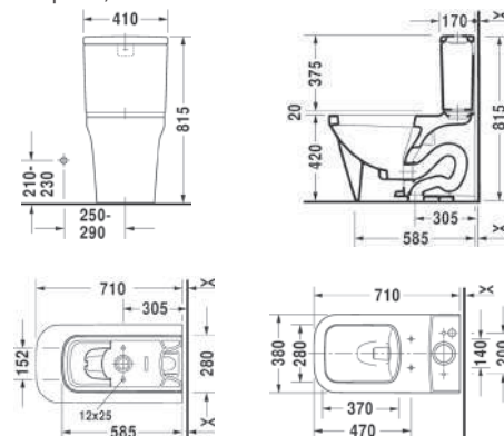
s/trap 305 mm toilet 216801 two-piece, rimless soft-close seat (option) 002059
